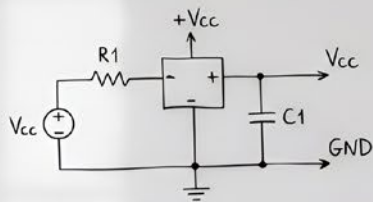
Power Supply Circuit Draft
